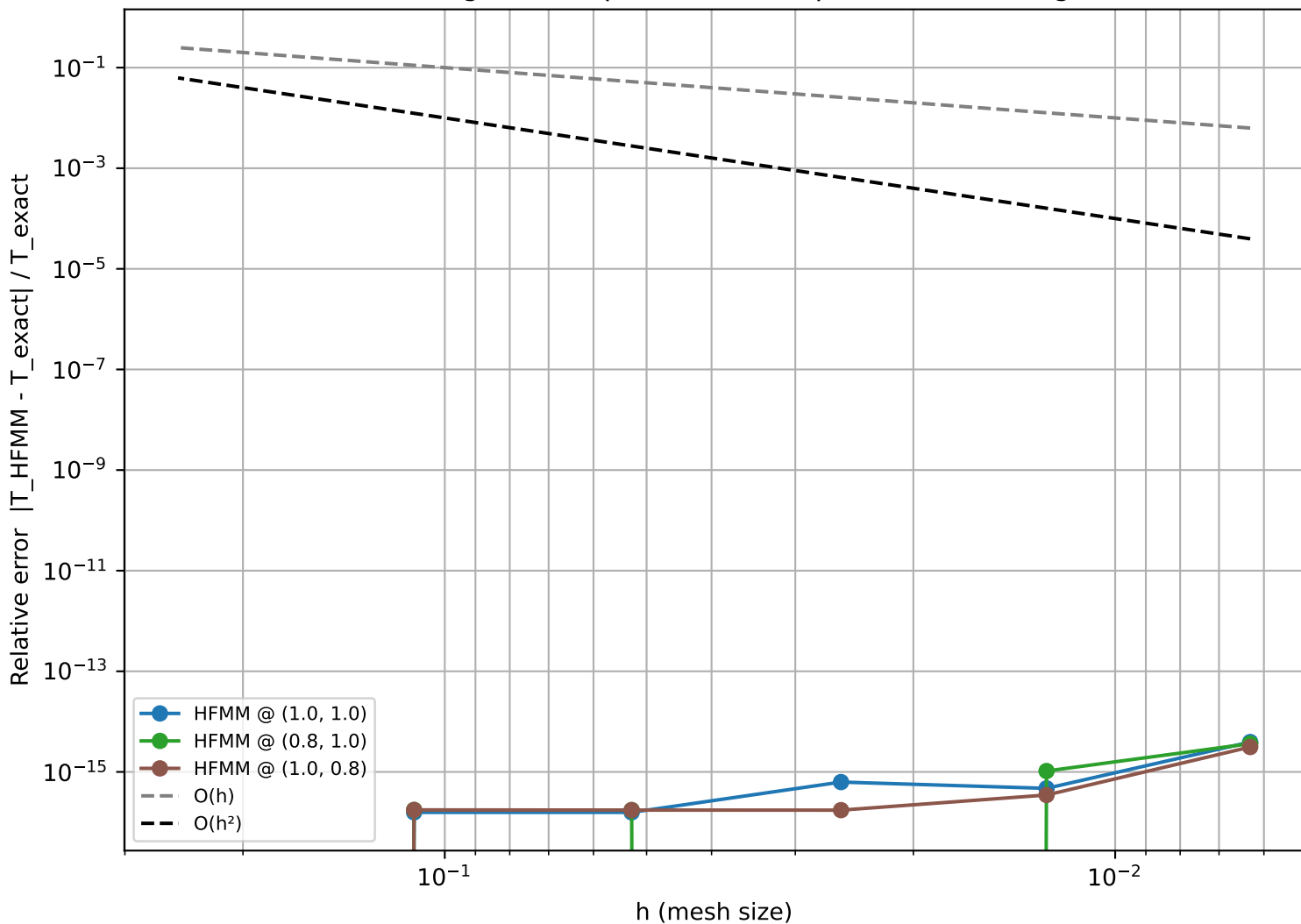
FMM Convergence - Square — HFMM pointwise convergence
